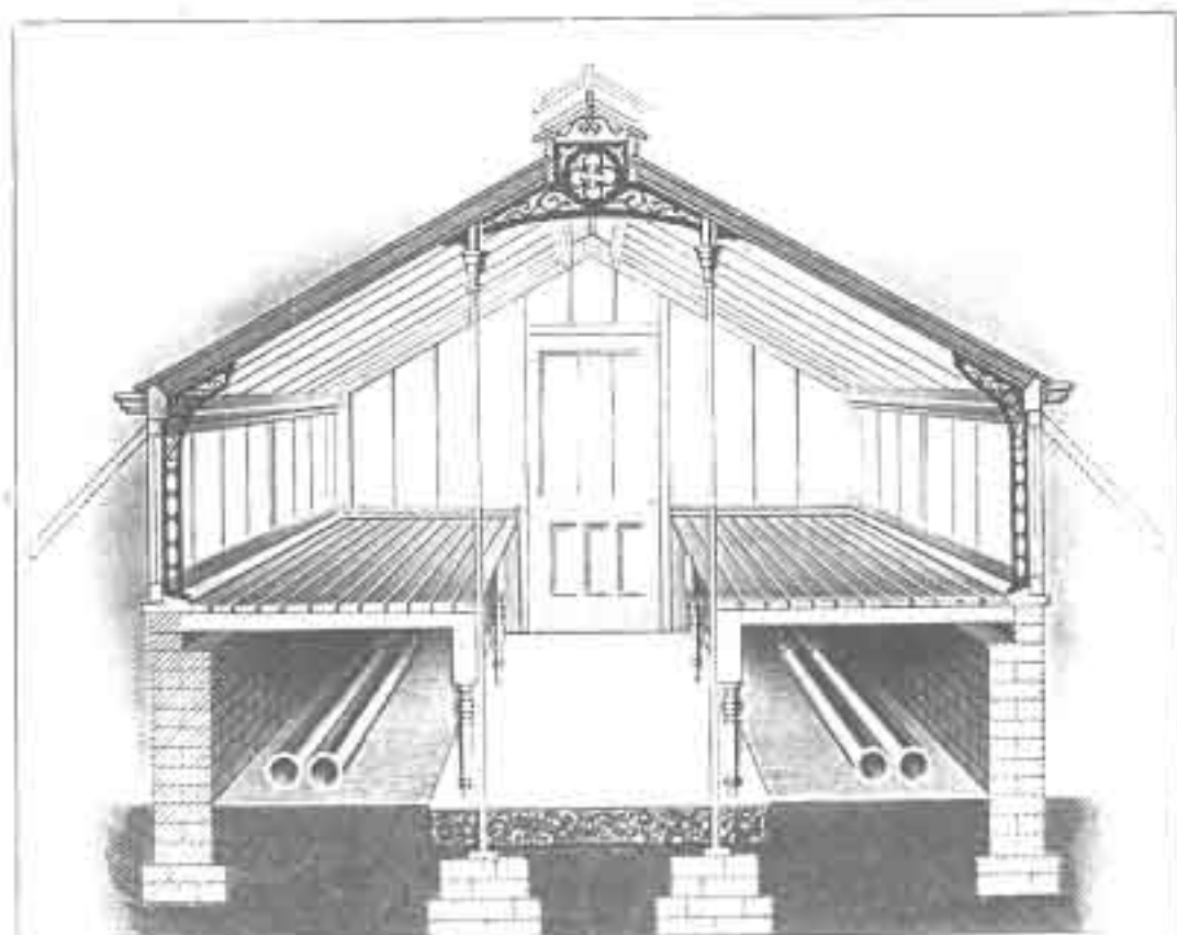
No. 54. SECTION OF SPAN PLANT HOUSE, 12 ft. wide, with lantern ventilation.
