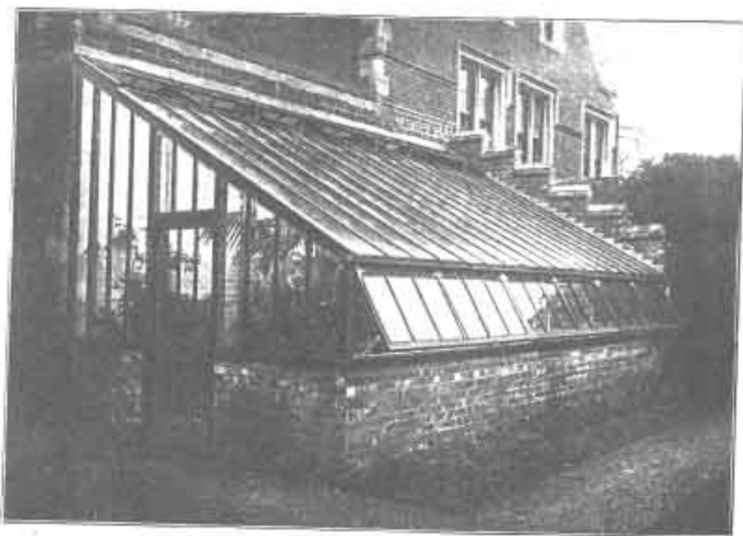
No. 65.—ELEVATION of LEAN-TO PLANT HOUSE, 12 ft. wide, on Brick Walls, erected in Teak for Major General Codrington, Preston Hall, Uppingham.
