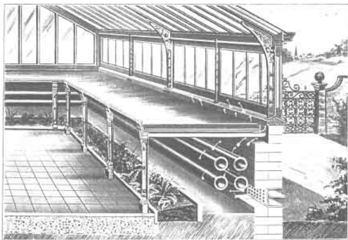
No. 59.—IRON STAGE FOR STOVES, etc., with Galvanised Iron Top; air admitted by our Registered Ventilators and passed over Pipes. These Stages are very durable and preserve a moist atmosphere round the plants.
