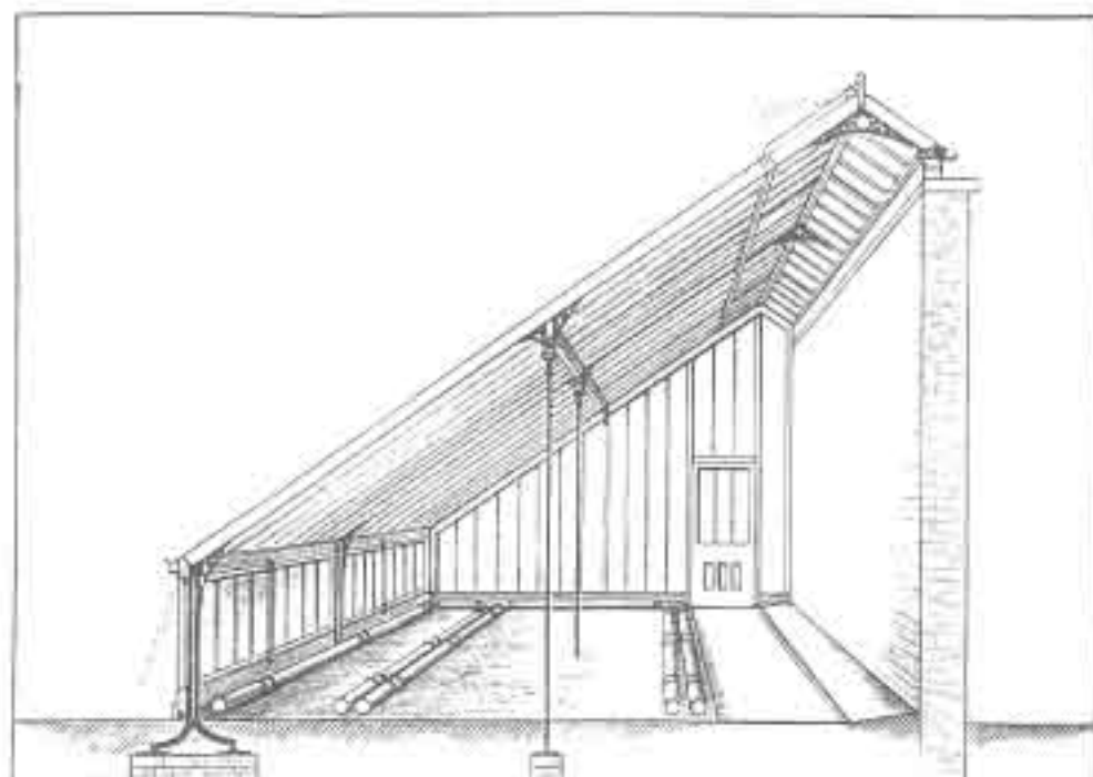
No. 75.—SECTION of THREE-QUARTER SPAN VINERY, 18 ft. wide, on F. & P.'s Iron Standards, for early forcing.
