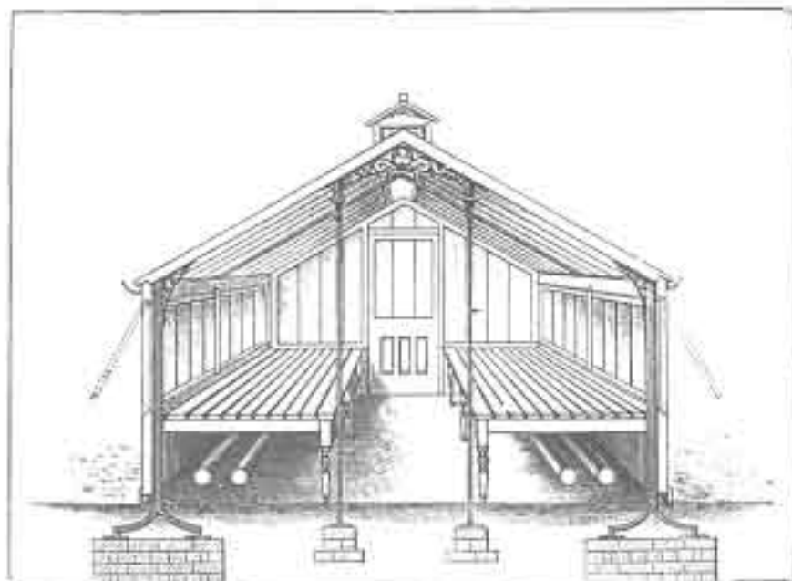
No. 56.—MOVABLE HOUSE ON IRON STANDARDS.
