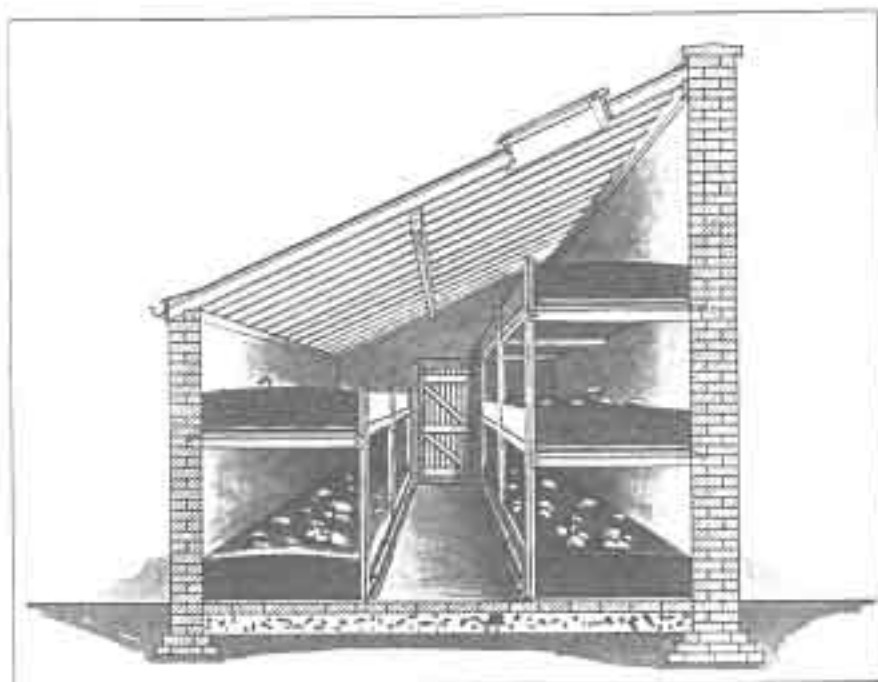
No. 90. SECTION OF MUSHROOM HOUSE, 12 ft. wide, erected for Earl of Zetland, Aske Hall, Richmond; also Carl Meyer, Esq., Shortgrove, Newport, Essex, and many others. The Shelves are formed of Slate Slabs resting on Cast-iron Frame. They give the largest space possible, and allow of the soil being readily removed.
