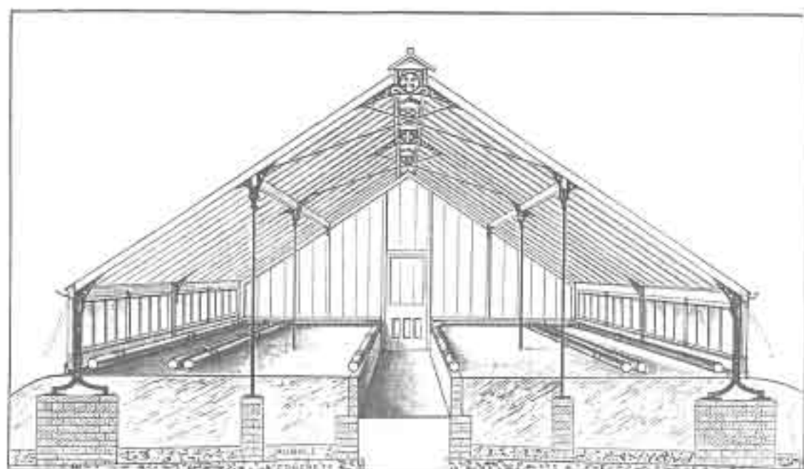
No. 74.—SECTION of SPAN VINERY, 25 ft. wide, on F. & P.'s Iron Standards, suitable for medium and late Houses, erected for the Right Hon. Lord Middleton, Birdsall, and others.
