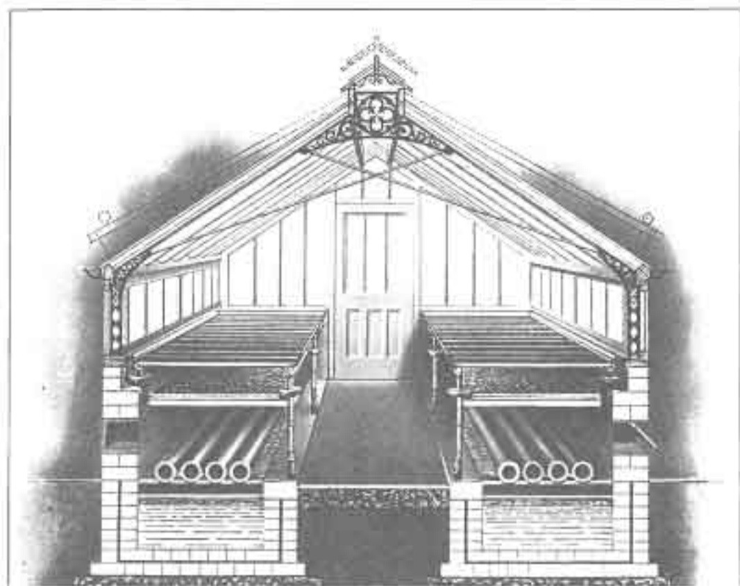
No. 50. SECTION of ORCHID HOUSE, 12 ft. wide, showing Improved Stages and Fittings, side Ventilation under Stage only, and top ventilation by our Improved Lantern.
