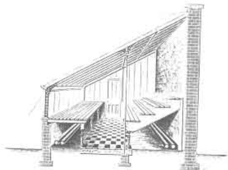
No. 64.—SECTION of LEAN-TO PLANT HOUSE, 12 ft. wide.
