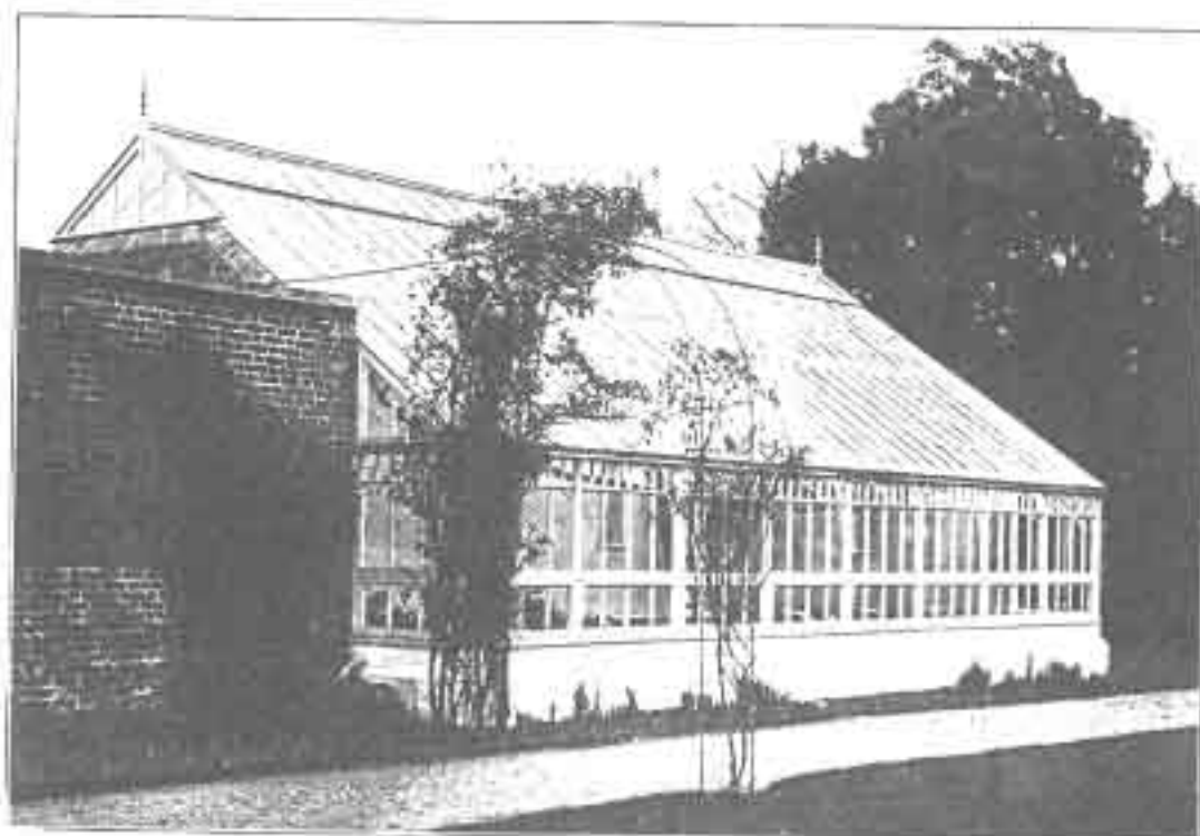
No. 16.—CONSERVATORY erected for Lady Esme Gordon, Paxton Park, St. Neots.
