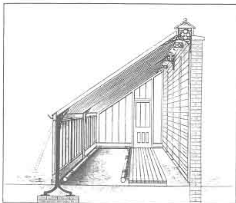
No. 78. — SECTION of PEACH HOUSE, 10 ft. wide, on F. & P.'s Iron Standards, with lantern top ventilation, resting on coping, erected at Feston Hall, Derbyshire, etc.
