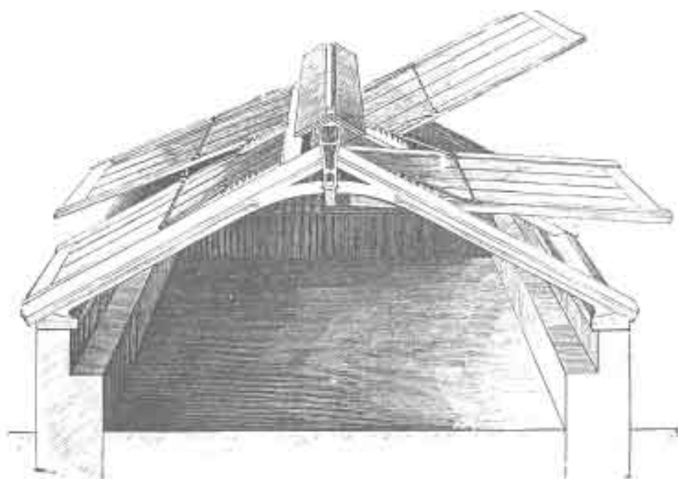
No. 82.—FRAME FOR FIXING ON BRICK WALLS, for Winter Vegetables and Plants requiring heat.
