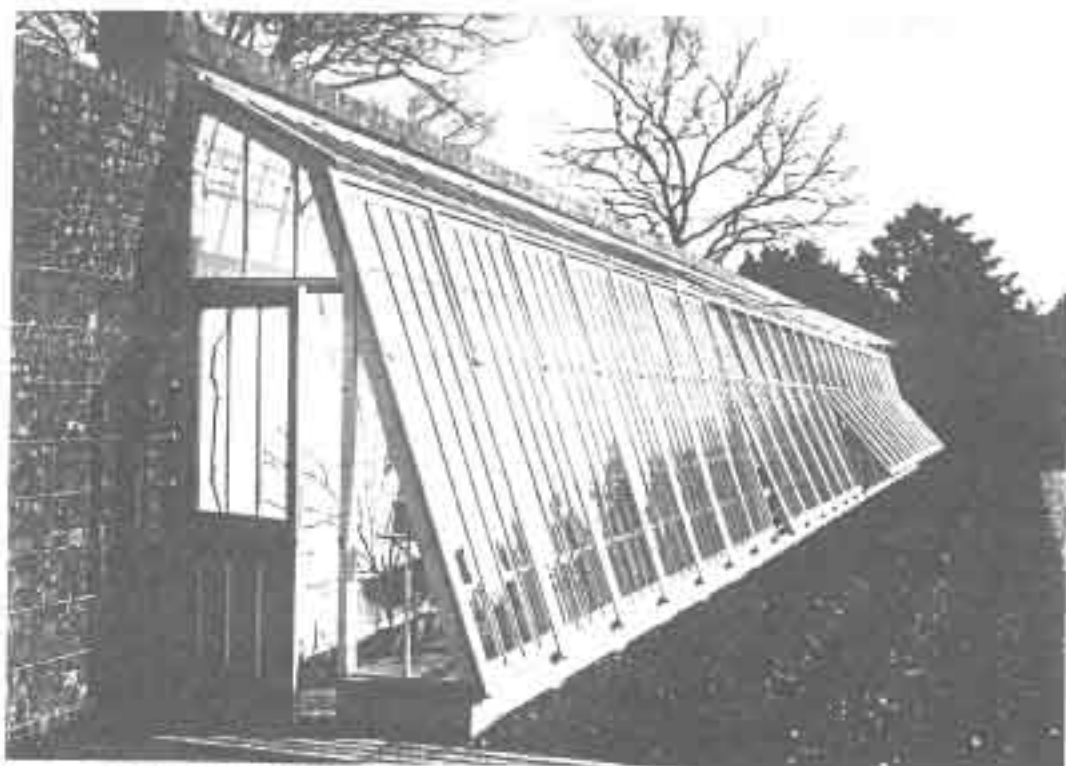
No. 79. — IMPROVED APRICOT and PEACH PROTECTOR, so constructed that all the lights can be removed. Erected for H. Bell, Esq., Mynthwest, Leigh, near Reigate, and many others.
