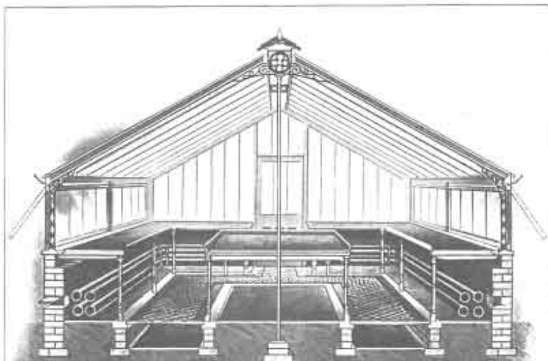
No. 52. —SECTION of CARNATION HOUSE, 18 ft. wide. Carnation Houses to this Section have been erected by us for Leopold de Rothschild, Esq., Ascott: W. D. James, Esq., West Dean, Chichester, etc.
