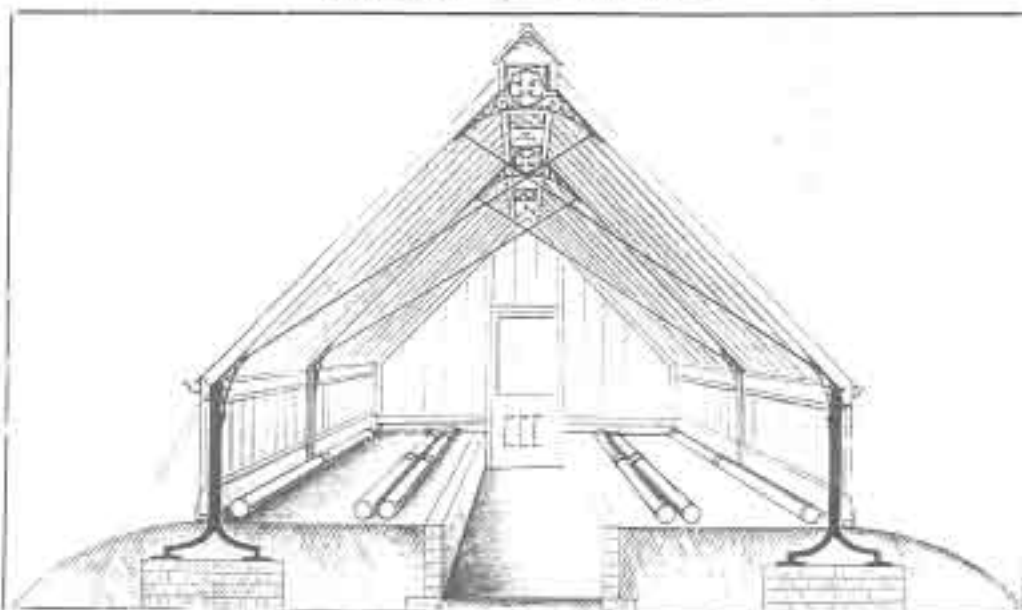
No. 71. SECTION OF VINERY, 14 feet to 16 feet wide, with square pitched roof, border 18 inches above floor level.
