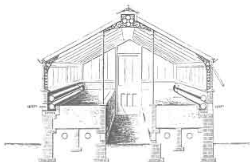
Section of Forcing House.
