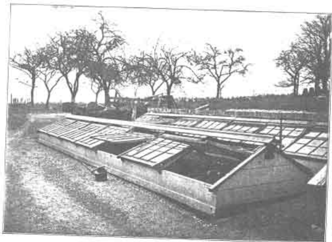
No. 81.—IMPROVED SPAN FRAME, 6 feet wide, as above. Erected for Sir A. S. Haslam, M.P., Breadsall Priory, near Derby.
