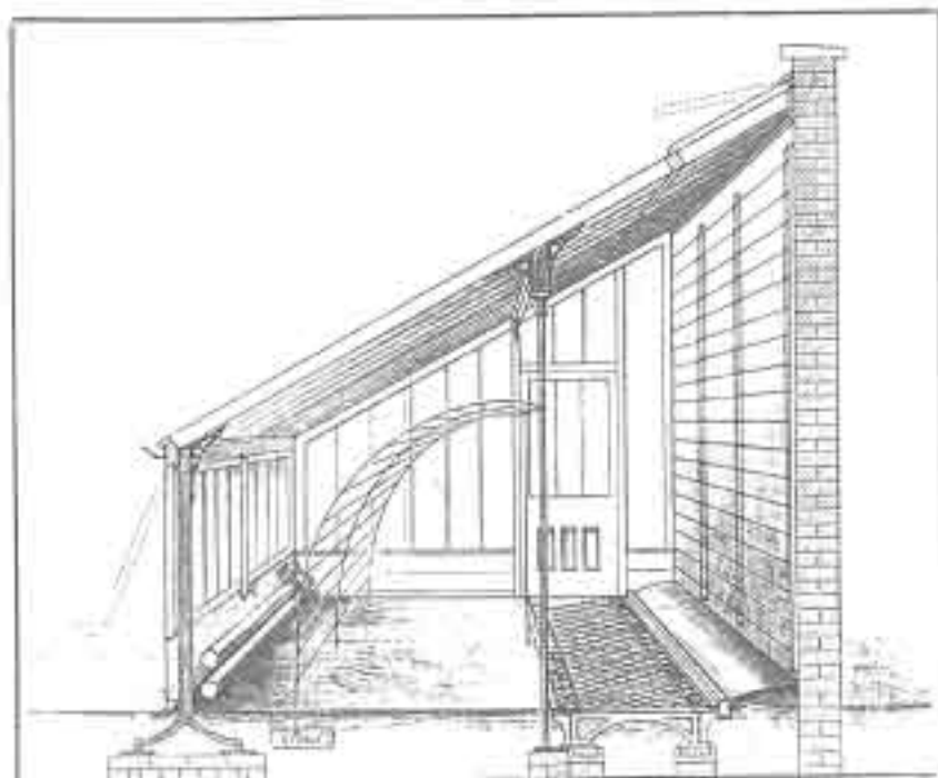
No. 76. SECTION of LEAN-TO PEACH HOUSE, 12 ft. wide, on F. & P.'s Iron Standards.
