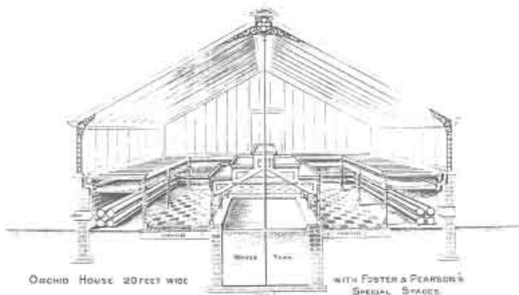
No. 51. SECTION of ORCHID HOUSE, 18 ft. or 20 ft. wide.
